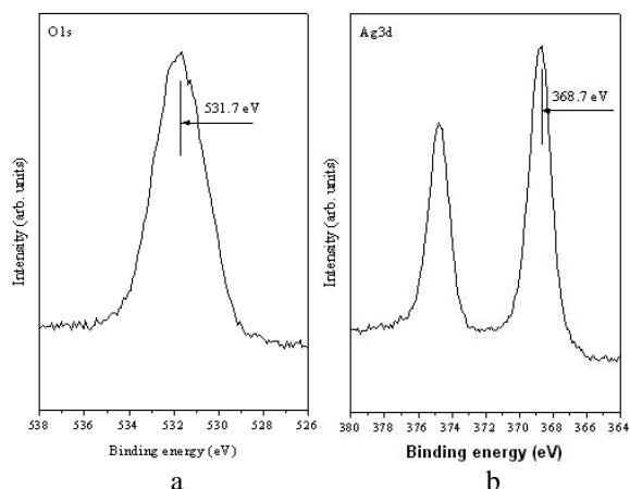
Fig. 2. The high-resolution photoelectron spectra of \text{O}1s (a), \text{Ag}3d (b) of the Ag-doped aluminium oxide coating deposited by magnetron sputtering method on the glass substrates
